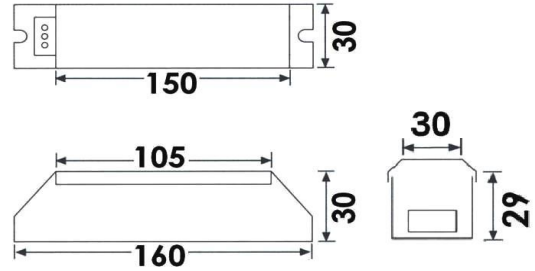
Dimensions (mm)
